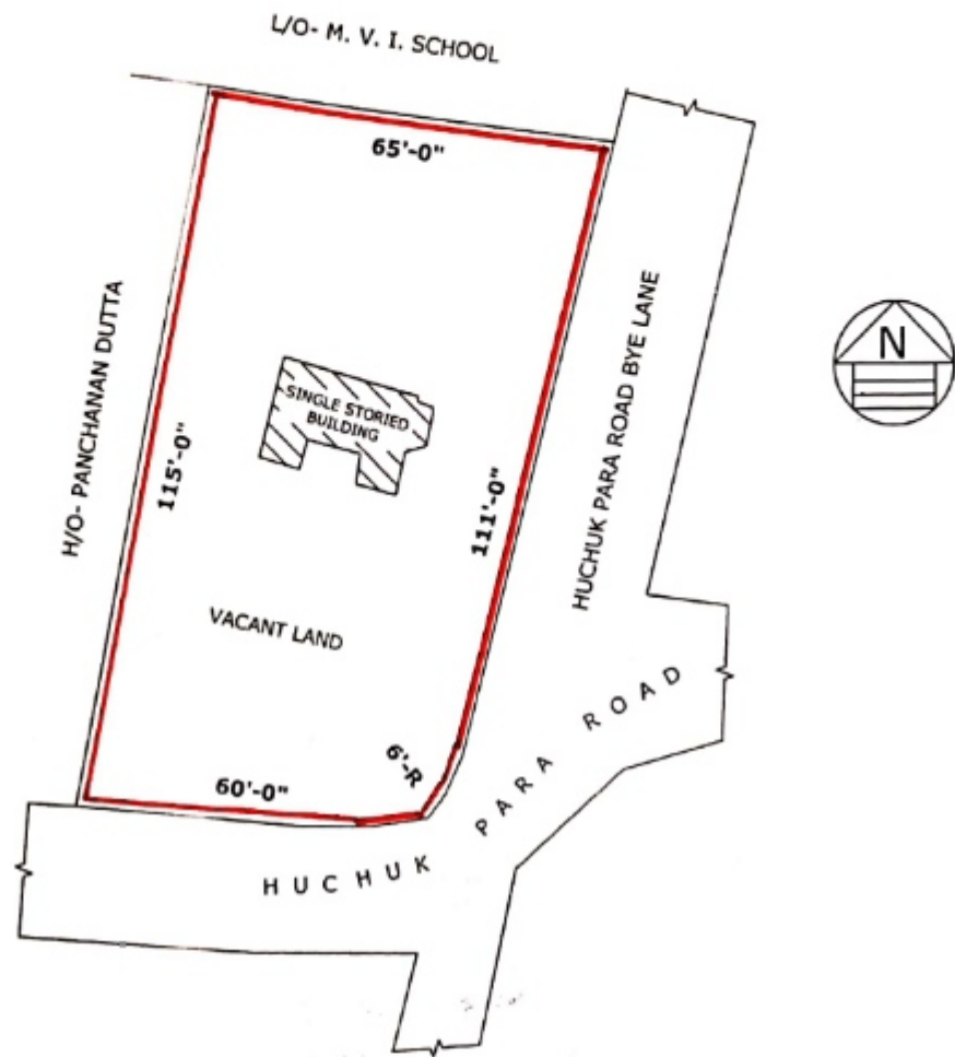
SITE PLAN SCALE : 16'-6"=1"
